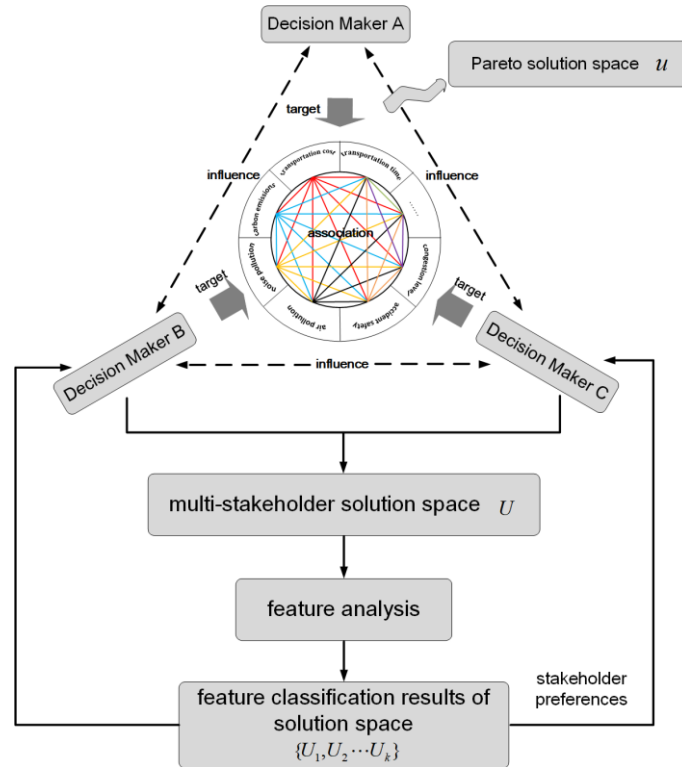
Figure 2: Approach to Solving the Multi-Stakeholder Pareto Stable Solution Set
