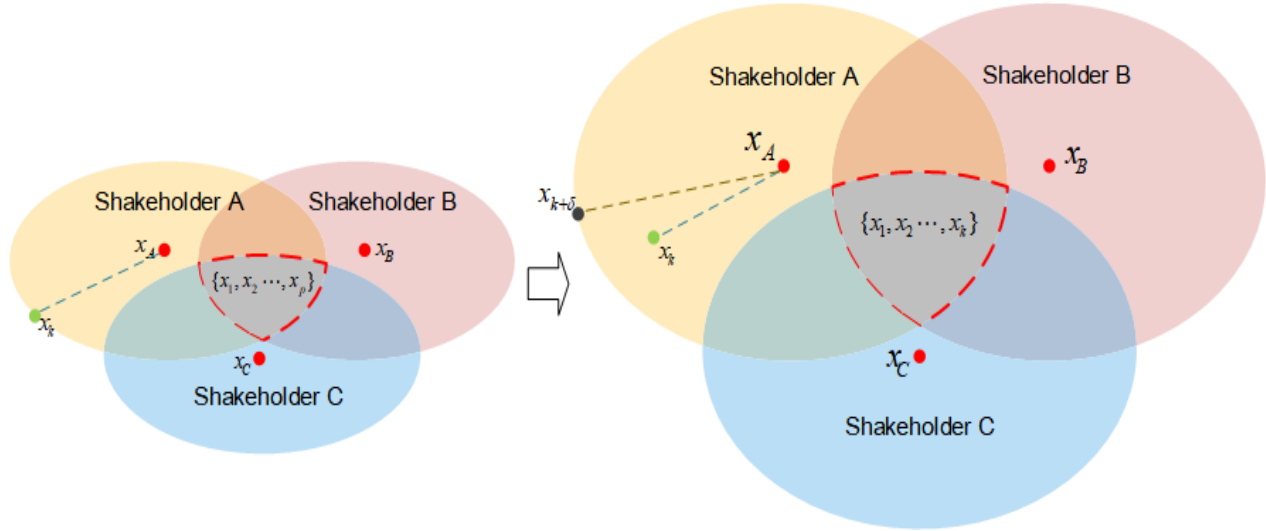
Figure 1: Multi-Stakeholder Pareto Stable Solution Set
