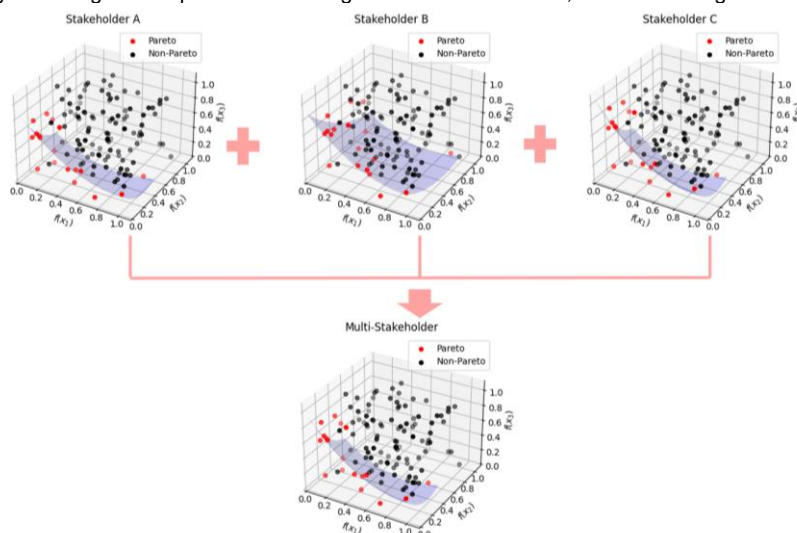
Figure 4 Construction of the Pareto Solution Space
