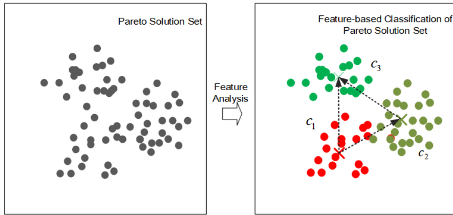
Figure 3 Structuring of the Pareto Solution Set
