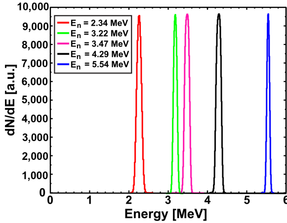
Figure 4: The calculated neutron energy spectra for the five experimental configurations are shown in Table 1.
