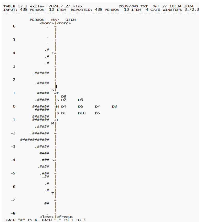
Figure 2: Results of the wright map.
