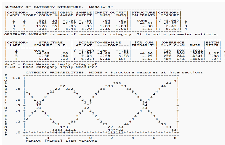
Figure 3: Probability curves for the four categories.
