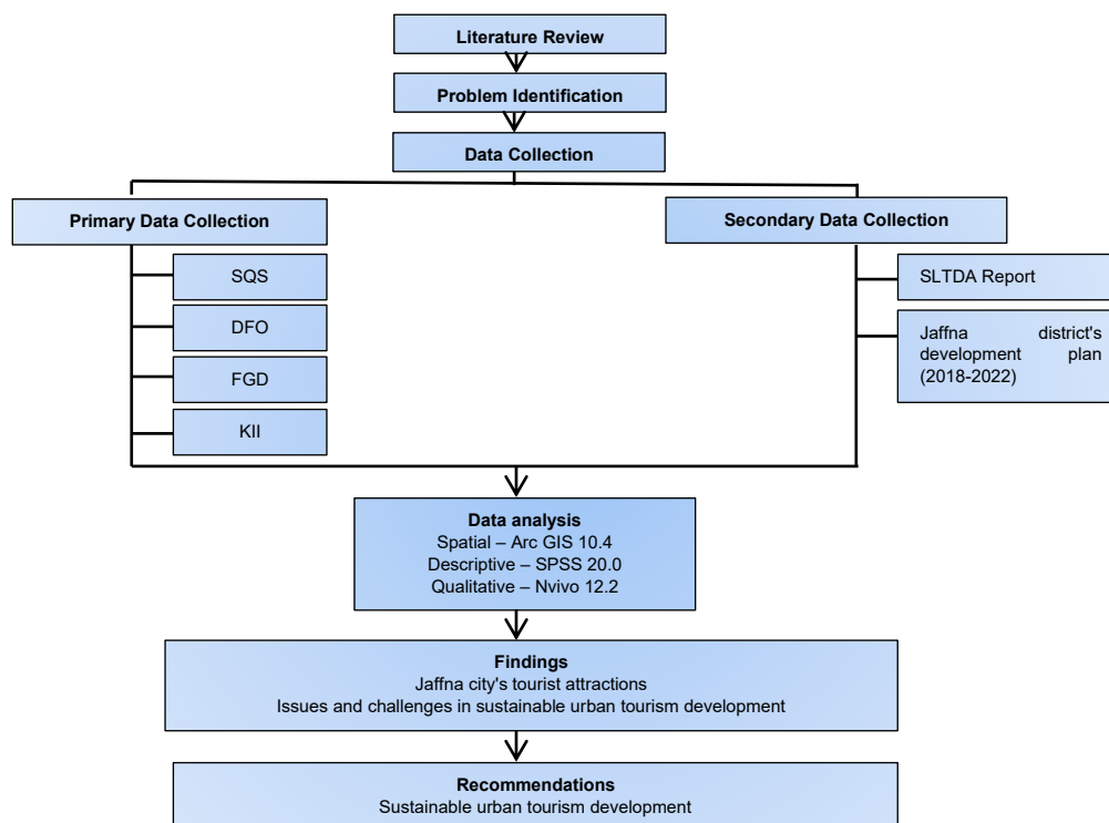
Figure 3: Methodological Framework
