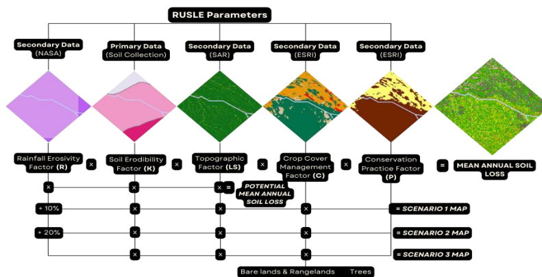
Figure 2. RUSLE conceptual framework.
