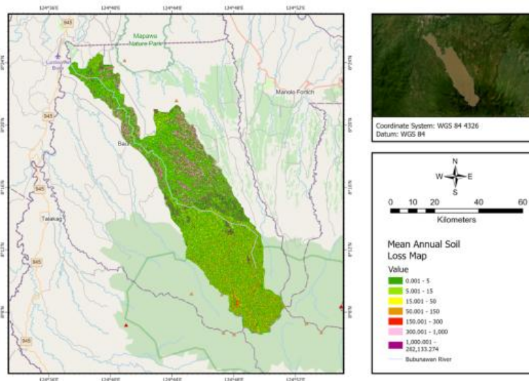
Figure 6. Mean annual soil loss map of the BRW.
