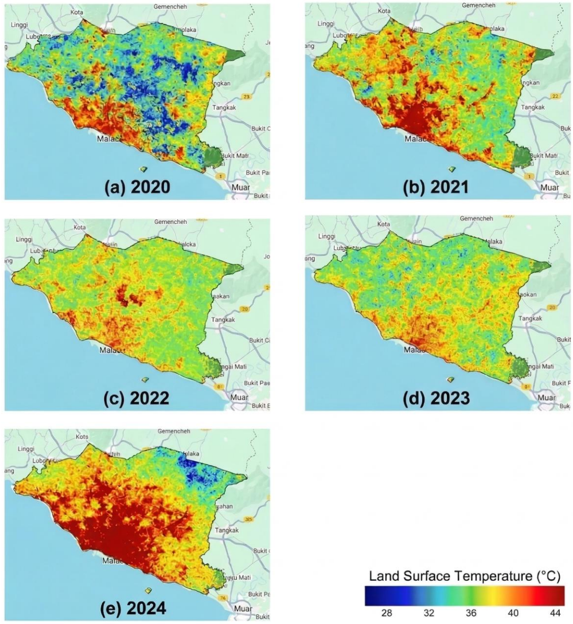
Figure 2: Spatial distribution of Land Surface Temperature (LST) in Melaka from 2020 to 2024. Source: Derived from Landsat 8 imagery using Google Earth Engine.
