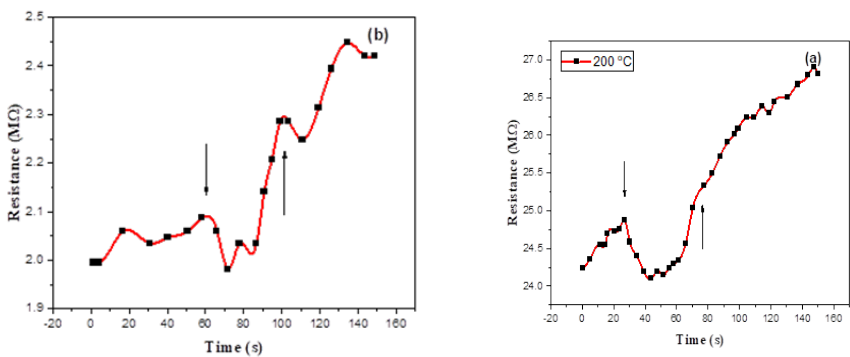
Figure 11: Resistance changes with time of GeO 2 :3 wt% SnO 2 thin film prepared with 350 mJ, for NH 3 gas (a) at 200°C, (b) at 250°C and (c) at 300°C. (continued on next page)
