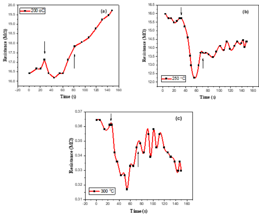
Figure 10: Resistance changes with time of GeO 2 :2 wt% SnO 2 thin film prepared with 350 mJ, for NH 3 gas (a) at 200°C, (b) at 250°C and (c) at 300°C.
