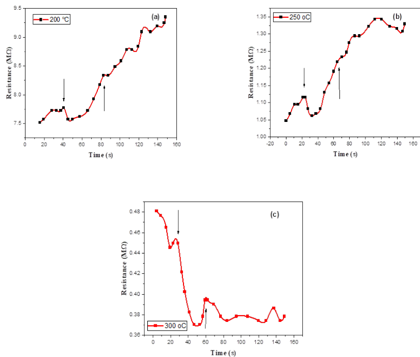
Figure 13: Resistance change with time of GeO 2 :8 wt% SnO 2 thin film prepared with 350 mJ, for NH 3 gas (a) at 200°C, (b) at 250°C and (c) at 300°C.
