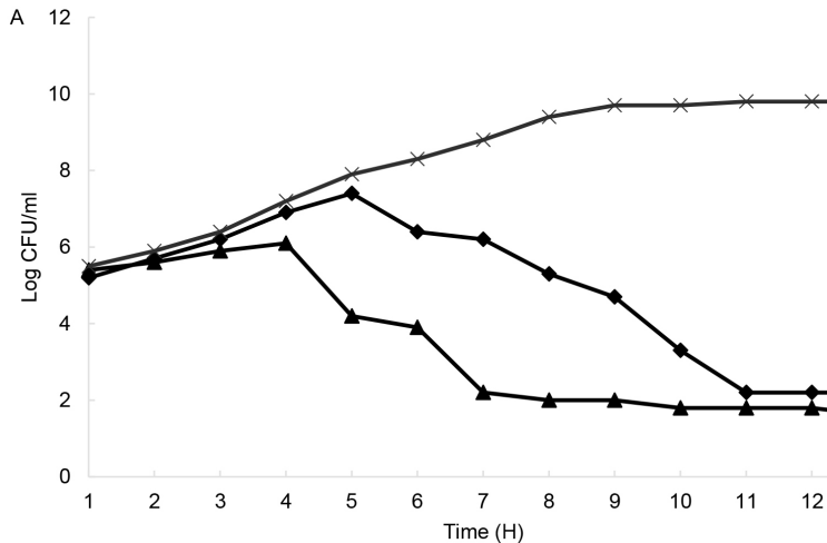
Figure 1: The kill curves of 2-octylcyclopentanone on (A) MRSA and (B) P. aeruginosa . The antimicrobial activity was concentration and time dependent. ( continue on next page )
