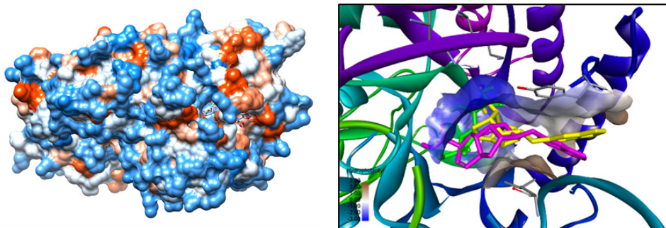
FIGURE 4: Compound 1 (yellow), 2 (pink) and D -saccharic acid 1,4-lactone (green) aligned in the binding pocket of \beta -glucuronidase protein in 3D structures.
