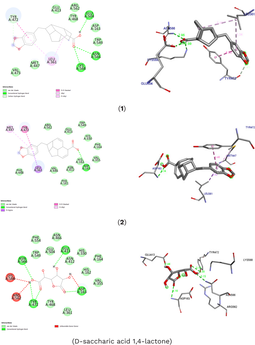
FIGURE 3: Illustration of 2D and 3D binding interactions of compound 1 , 2 and D-saccharic acid 1,4-lactone with \beta -glucuronidase protein.
